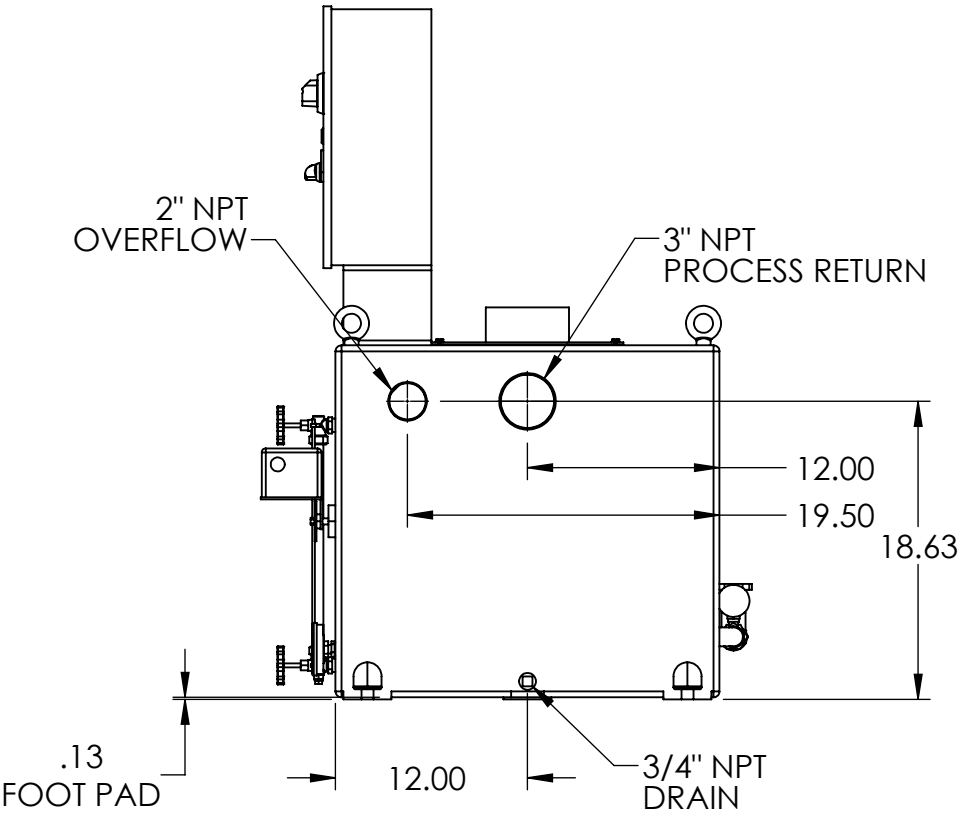
BACK VIEW
